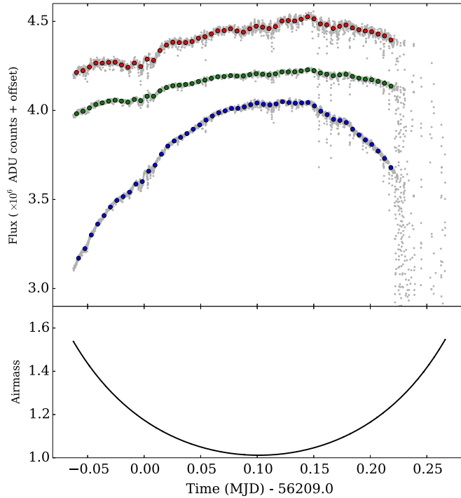
Figure 5.4: Raw light curves for WASP-33 in the red, green and blue channels. The grey points are the unbinned raw fluxes, while the coloured points are the binned versions of the sigma-clipped fluxes (with the final hour of data also removed). The effect of clouds in the final hour of the observations is clear. Shorter time-scale variations in the raw flux are suggestive of passing cirrus cloud. The long time-scale curvature in these light curves is a result of atmospheric extinction, which correlates with the airmass (shown in the bottom panel).
