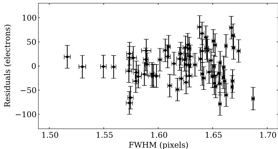
Figure 3.16: Channel 1 flux residuals plotted against the FWHM (using Gaussian profile fitting centroiding method). The residual and FWHM values were binned (in time) at the same level as in Figure 3.12 before being plotted. There is no clear trend in the residuals with FWHM, suggesting that variations in the FWHM are not causing the residual systematic variations in channel 1.
