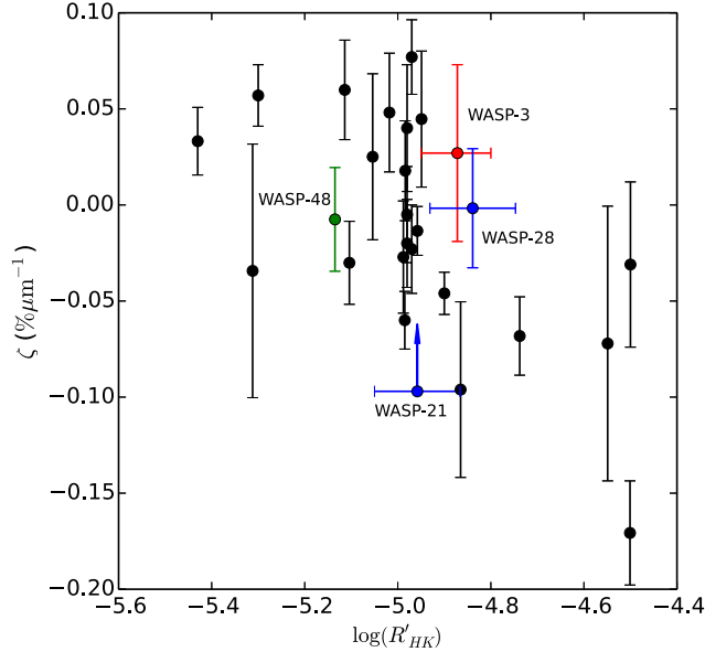
Figure 4.25: The correlation between \log R'_{\text{HK}} and \zeta as presented in Figure 3.21, but here with additional measurements for WASP-21 and WASP-28 (plotted as blue points). No reliable \log R'_{\text{HK}} measurement exists for WASP-37. The errors on \log R'_{\text{HK}} for WASP-21 and WASP-28 reflect the errors on a single measurement, rather than the range of values found over a few years, as is the case for WASP-3 (highlighted in red). Like WASP-3, WASP-28 orbits a moderately active star, but does not seem to have strong absorption in the 4.5 \mu\text{m} band (IRAC channel 2) - its \zeta value is consistent with a blackbody. This object, along with WASP-48 (highlighted in green) is discussed in the text. With the addition of the data for WASP-28 and WASP-48, the Pearson correlation coefficient here is r = -0.58 , suggesting little change from the value of r = -0.59 found in Section 3.5.3.
