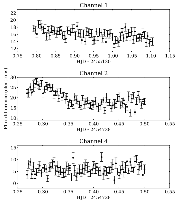
Figure 3.8: Figure showing difference in photometry between using my chosen background estimation method ( 4\sigma clipped mean) and a median. For comparison the eclipse depths are 150^{+30}_{-20} , 650 \pm 30 and 160^{+40}_{-30} electrons for channels 1, 2 and 4 respectively. Offsets in flux will have a negligible effect on the eclipse depth, but changes to these flux differences could impact the results. However, the largest variation, seen in channel 2, is still at only 0.3\sigma of the final eclipse depth. Hence the differences between different background estimation methods are insignificant.
