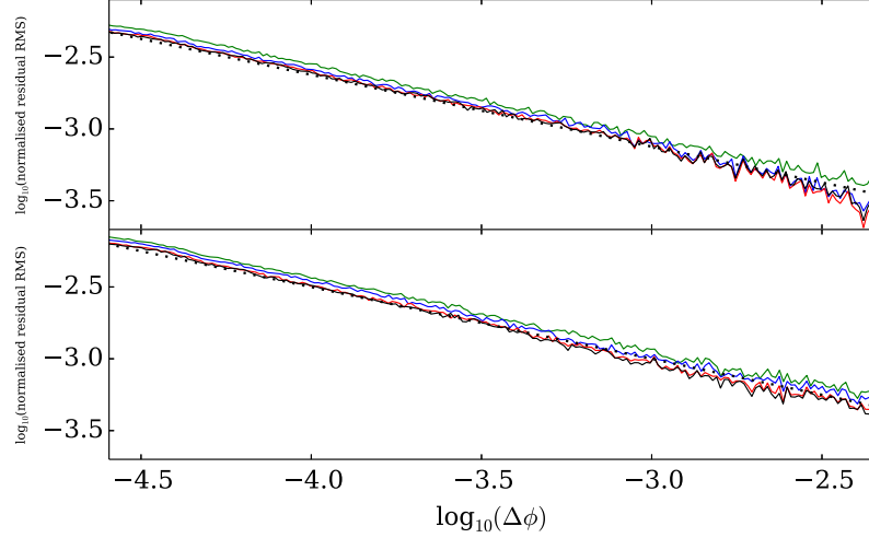
Figure 4.14: An equivalent plot to Figure 4.7, but here shown for the WASP-28 channel 1 and 2 data. In both channels, the binned RMS values follow the white noise expectation down to the largest bin sizes.
