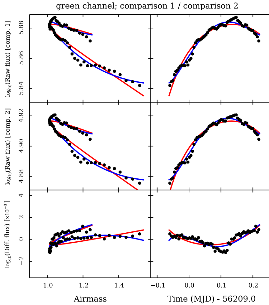
Figure A.1: Equivalent plot to Fig. 5.7, but here given for the green channel of ULTRACAM. The variations in the differential flux light curve seen in the red channel are also seen here.
