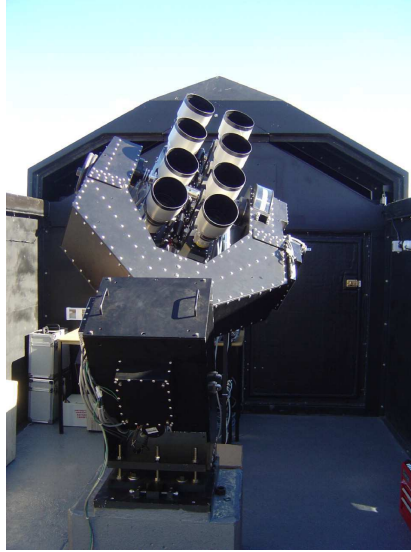
Figure 1.6: One of the two SuperWASP instruments [Pollacco et al., 2006], here shown at the South African Astronomical Observatory.
