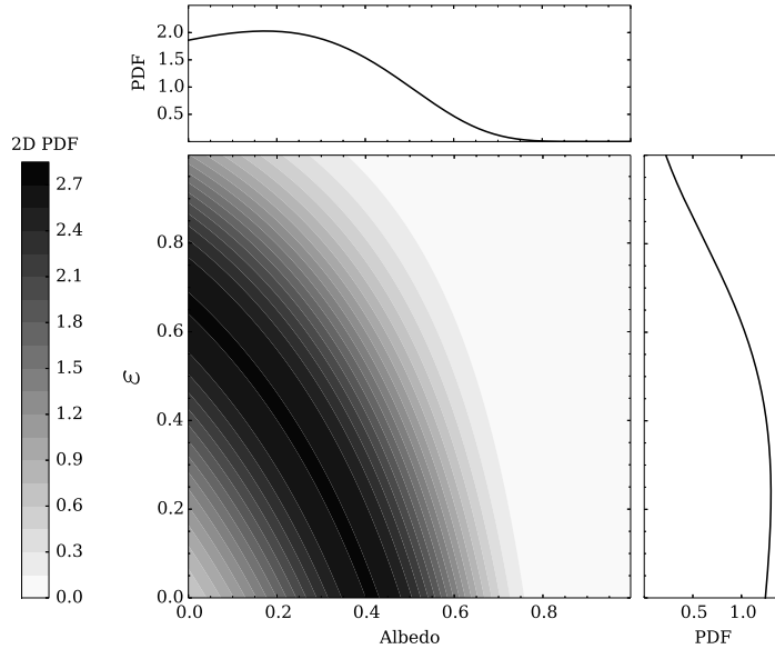
Figure 3.18: A probability distribution found using my T_d/T_0 value with equation 2.39, assessed over a grid of allowable albedo and \varepsilon values. Darker regions are of higher probability than lighter regions. The resulting distribution shows the ambiguity between the albedo and heat redistribution parameters, where a low albedo with a moderate \varepsilon reproduces T_d/T_0 equally as well as a moderate albedo with a low \varepsilon . Also shown are the marginalised PDFs for the two parameters.
