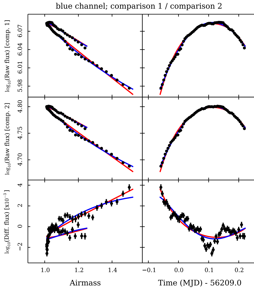
Figure A.2: Equivalent plot to Figs. 5.7 and A.1, but here given for the blue channel of ULTRACAM. The differential flux variation seen in the red and green channels is present, with an additional trend due to the colour difference of comparison 1 and comparison 2.
