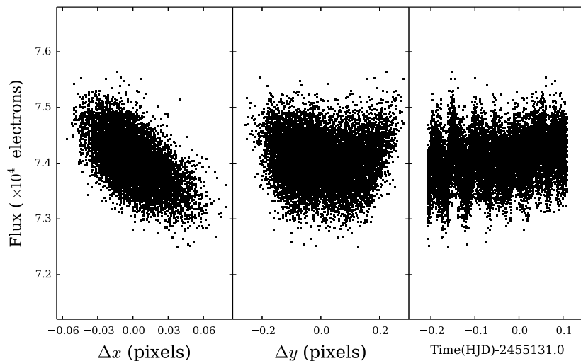
Figure 3.9: A plot of the channel 1 raw flux against dx and dy position and also against time. dx = x - \hat{x} and dy = y - \hat{y} are the positions of the PSF centre relative to their weighted means. There is a clear correlation between the flux and x position, while in y the PSF crosses a pixel boundary, where the minimum of the intra-pixel sensitivity function is sampled. A slight u-shape can be seen in the middle panel however. The trend of flux in time shows the typical \sim 1\% variations on a \sim 1 hr timescale.
