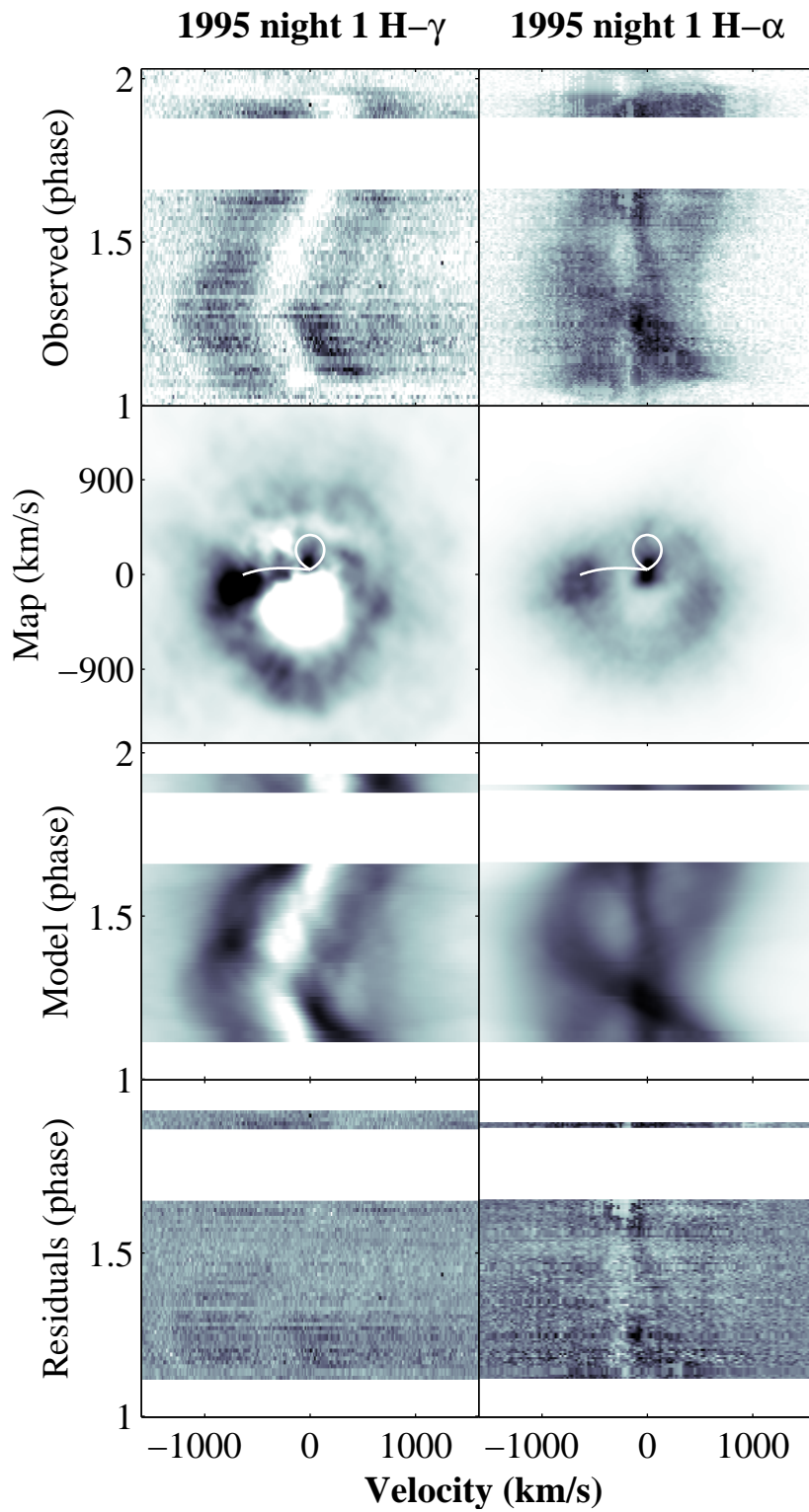
Figure 5.11: Trailed data, doppler maps, computed trail and residuals for the first night in 1995. See text for details.
