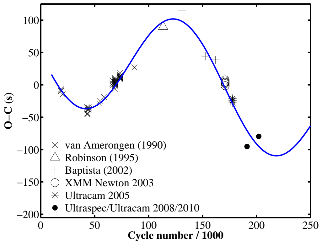
Figure 6.12: The new ephemeris O-C, generated from previous data, ten XMM OM eclipses, six Ultracam eclipses, and an Ultraspes eclipse.
