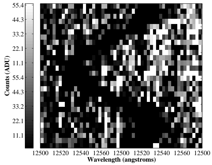
Figure 7.4: Trail of the KI line in X-Shooter OY Car data.
