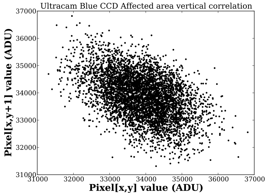
Figure 8.10: The vertical pixel correlation in a peppered area of the blue CCD.
