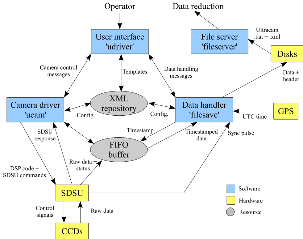
Figure 4.2: A schematic of the flow of information in the Ultracam software stack with endpoints meeting the hardware and end-user.
