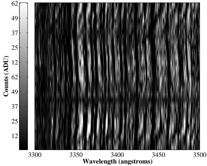
Figure 7.8: A portion in wavelength of the trailed OY Car data in the UV arm from X-Shooter. All the absorption lines seen can be attributed to iron.
