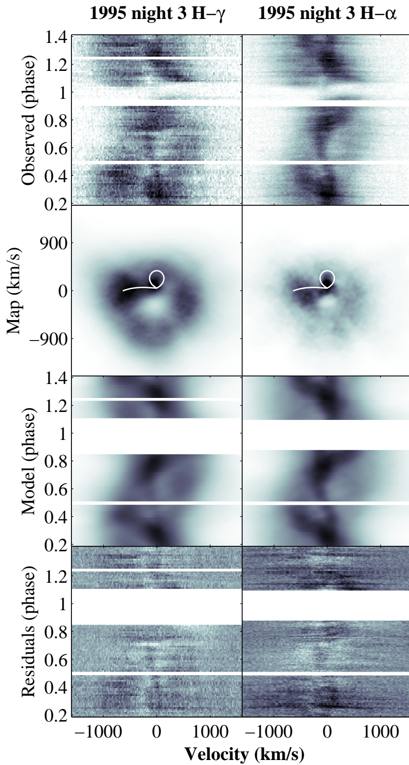
Figure 5.13: Trailed data, doppler maps, computed trail and residuals for the third night in 1995. See text for details.
