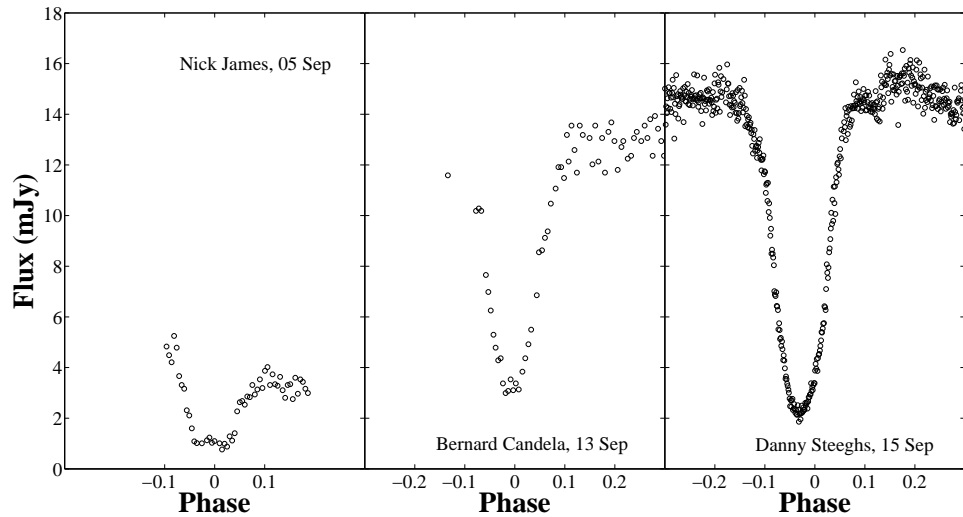
Figure 5.5: Optical V-band data taken with amateur telescopes and the 0.9m James-Gregory telescope (right) leading up to and after the HST run.
