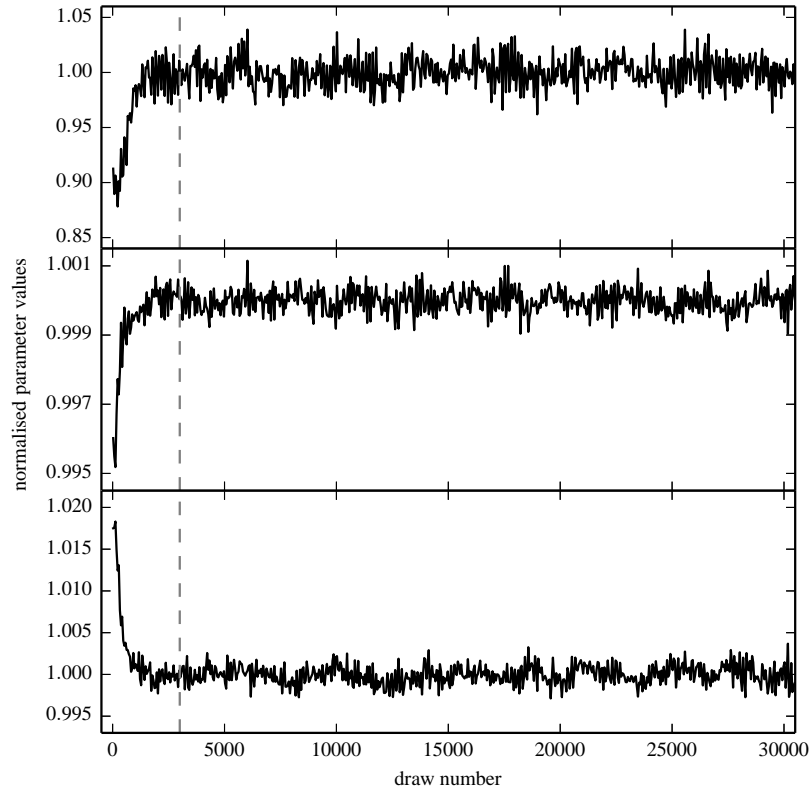
Figure 2.9: Normalised parameter values as a function of the number of draws in a Markov chain Monte Carlo simulation to illustrate convergence of the chain and the warm-up phase (to the left of the vertical dashed line).
