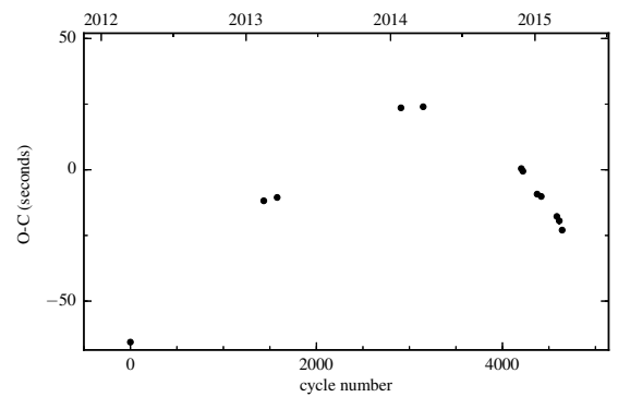
Figure B.24: O-C diagram of SDSS J1028+0931.
