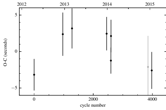
Figure B.19: O-C diagram of SDSS J0946+2030.
