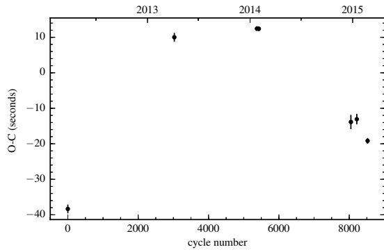
Figure B.25: O-C diagram of SDSS J1057+1307.
