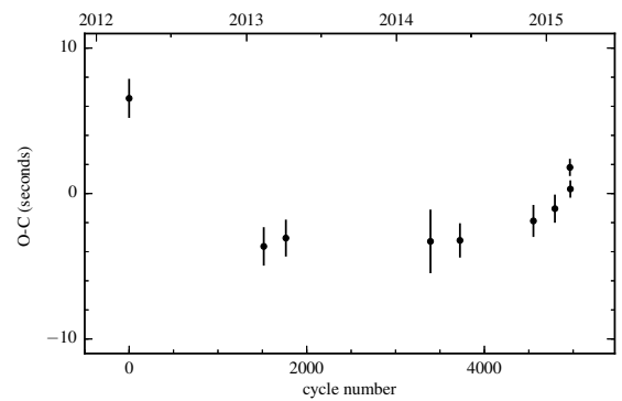
Figure B.30: O-C diagram of SDSS J1307+2156.
