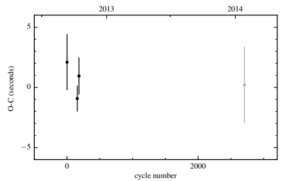
Figure B.6: O-C diagram of SDSS J0308-0054.
