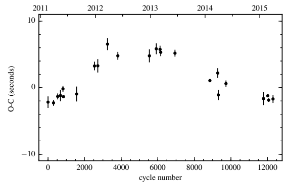
Figure B.34: O-C diagram of WD 1333+005.
