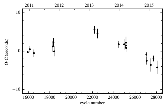
Figure B.12: O-C diagram of CSS 40190.
