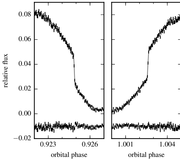
Figure 6.6: Data as in Fig. 6.5, with my best lcurve model over-plotted (light grey lines), corresponding to an inclination i = 87^\circ . The residuals are shown as well (vertically offset by -0.01).
