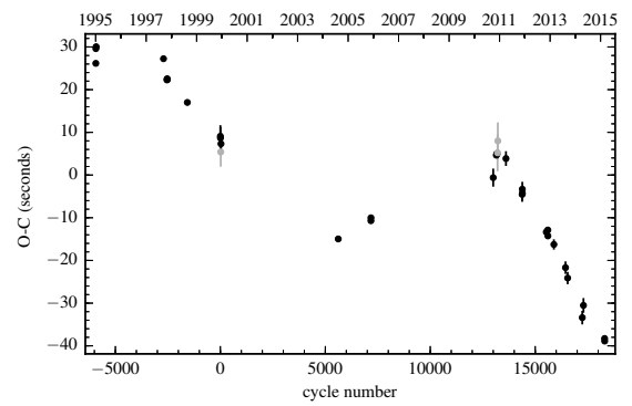
Figure B.10: O-C diagram of RR Cae.
