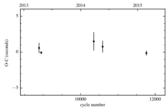
Figure B.42: O-C diagram of SDSS J1424+1124.
