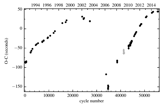
Figure B.36: O-C diagram of QS Vir.
