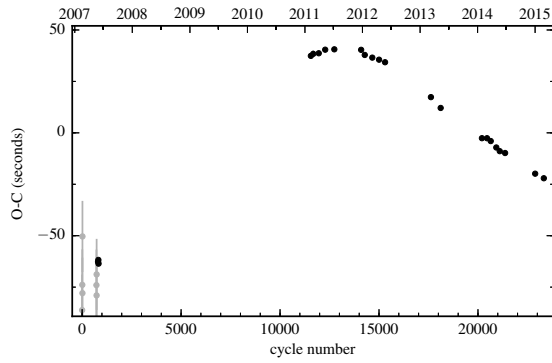
Figure B.43: O-C diagram of SDSS J1435+3733.
