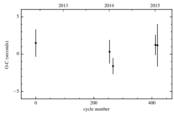
Figure B.16: O-C diagram of SDSS J0927+3329.
