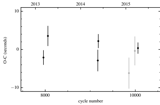
Figure B.37: O-C diagram of CSS 07125.
