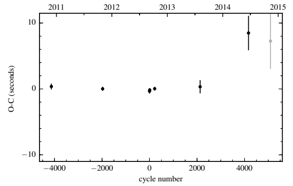
Figure B.50: O-C diagram of CSS 09704.
