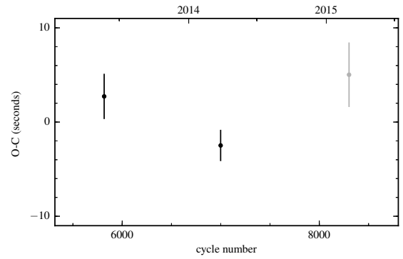
Figure B.44: O-C diagram of SDSS J1540+3705.
