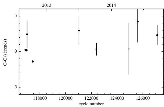
Figure B.59: O-C diagram of EP Dra.
