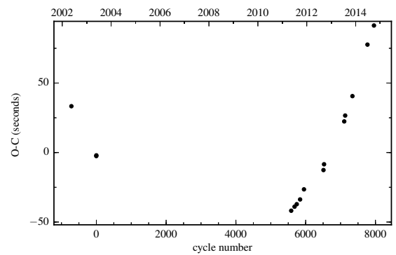
Figure B.48: O-C diagram of RX J2130.6+4710.
