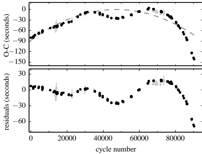
Figure 6.10: O-C diagram of the mid-egress times of HU Aqr including the best quadratic fit as the dashed grey line (top panel), and the residuals relative to that fit (bottom panel). O-C times with uncertainties exceeding 3 seconds have been greyed out for clarity, but all data were used to obtain the fit.
