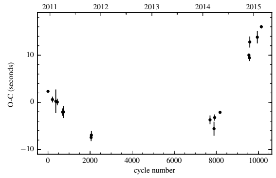
Figure B.20: O-C diagram of CSS 41631.
