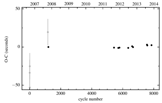
Figure B.2: O-C diagram of SDSS J0110+1326.
