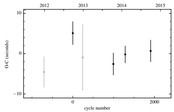
Figure B.4: O-C diagram of PTFEB28.235.
