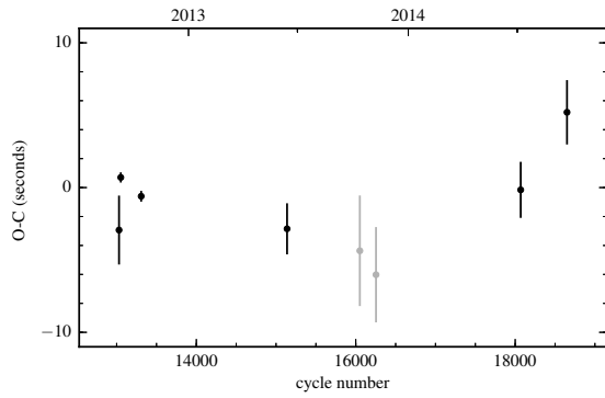
Figure B.49: O-C diagram of SDSS J2205-0622.
