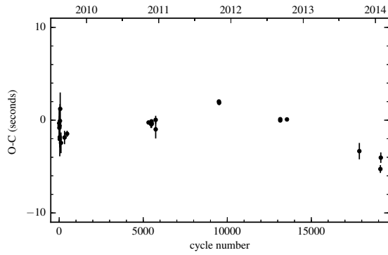
Figure B.1: O-C diagram of SDSS J0106-0014.
