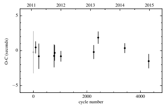
Figure B.18: O-C diagram of CSS 38094.
