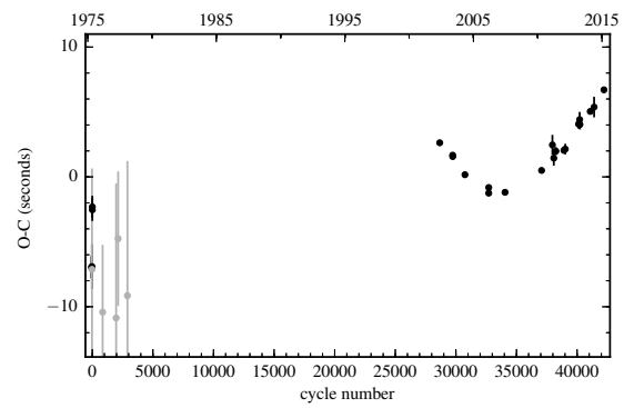
Figure B.40: O-C diagram of GK Vir.
