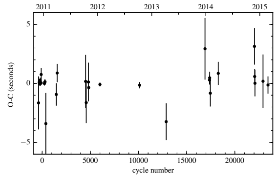
Figure B.14: O-C diagram of CSS 03170.
