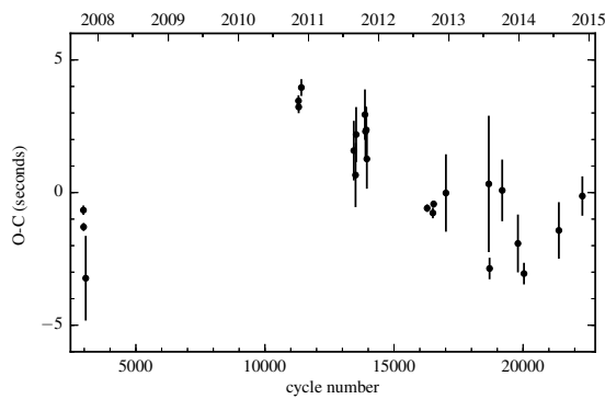
Figure B.5: O-C diagram of SDSS J0303+0054.
