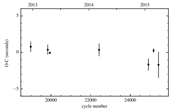
Figure B.22: O-C diagram of SDSS J1013+2724.
