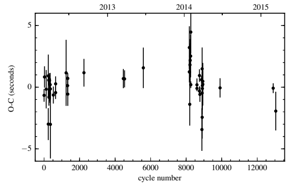
Figure B.38: O-C diagram of CSS 21055.
