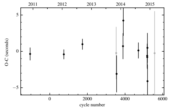
Figure B.8: O-C diagram of NLTT 11748.
