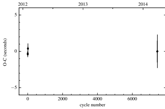
Figure B.13: O-C diagram of SDSS J0857+3318.
