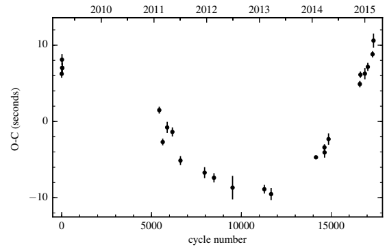
Figure B.26: O-C diagram of SDSS J1210+3347.
