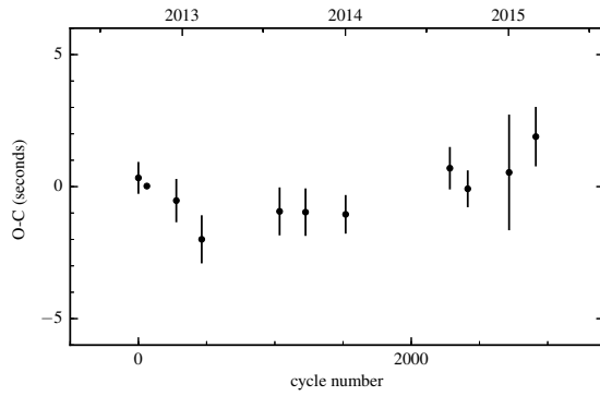
Figure B.7: O-C diagram of SDSS J0314+0206.
