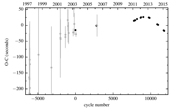
Figure B.32: O-C diagram of DE CVn.
