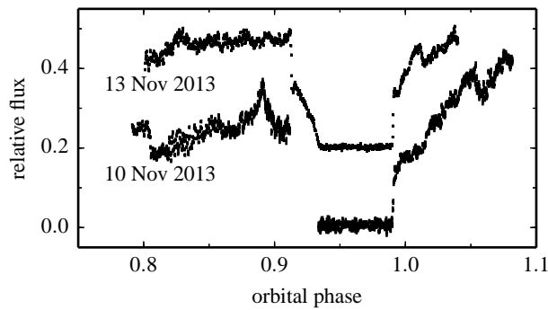
Figure 6.3: TNT+ULTRASPEC light curves of HU Aqr, taken in November 2013, displayed with a vertical offset of 0.2. To calculate the orbital phase I used the ephemeris from equation 6.2.
